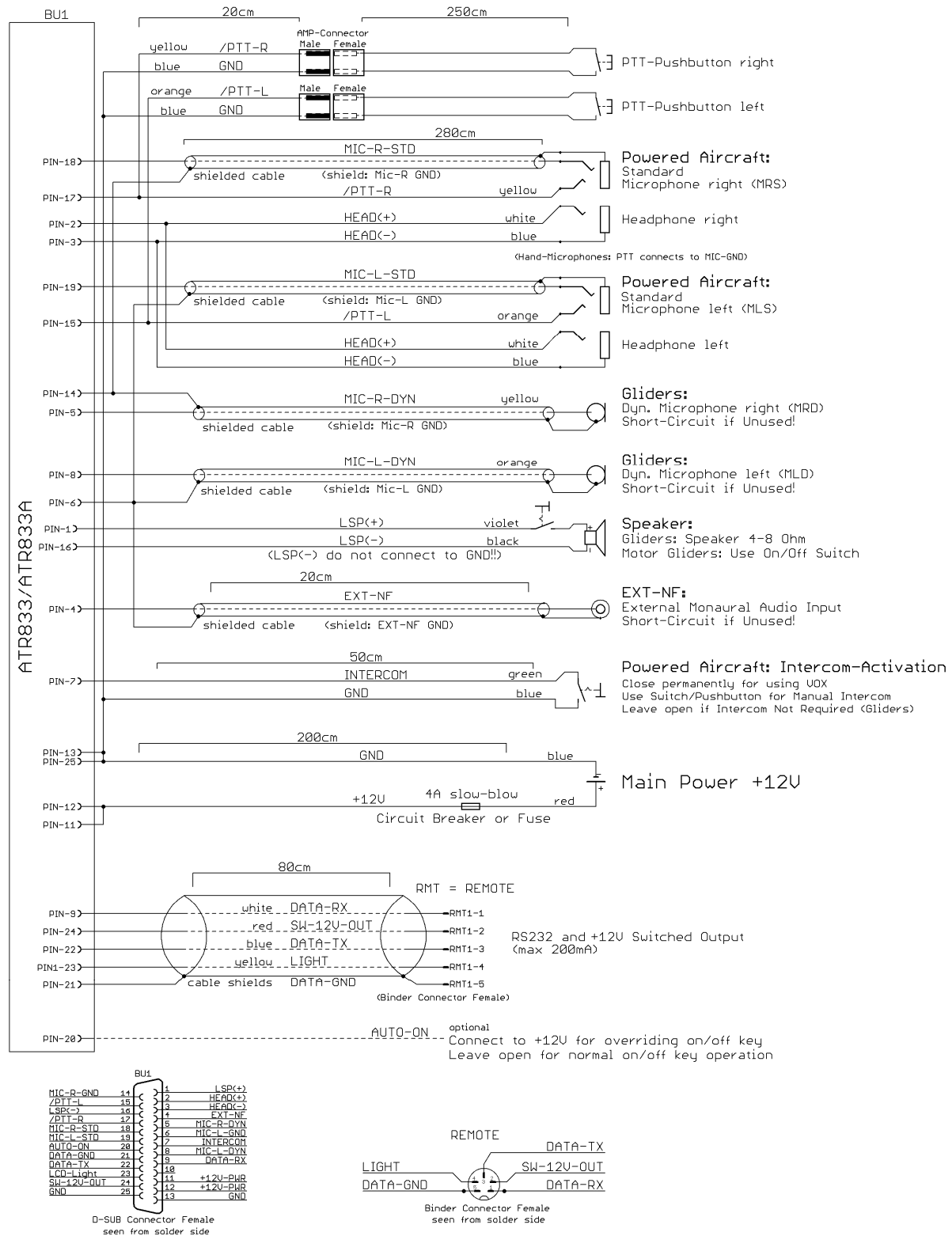
Cable ATR833/ATR833A
